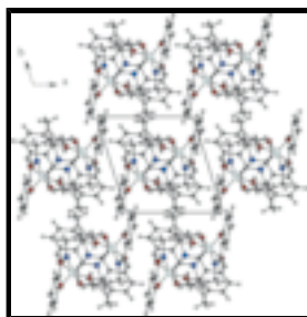
Fig. 3. Packing plot of (I) along [001].
