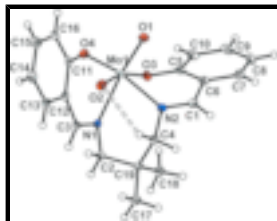
Fig. 1. Molecular structure of (I), with displacement ellipsoids drawn at the 50% probability level. H atoms are shown as circles of arbitrary radius. Hydrogen bonds are represented as dotted lines.
